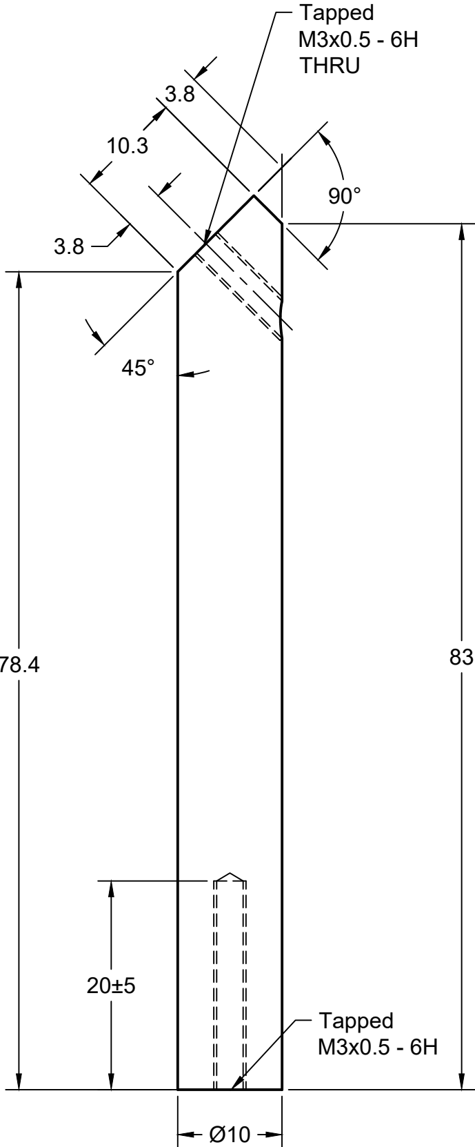
RIGHT VIEW
